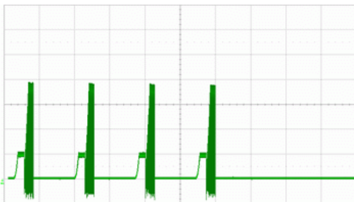
Locked rotor current at 24 V; 0,5A/div; 10s/div
