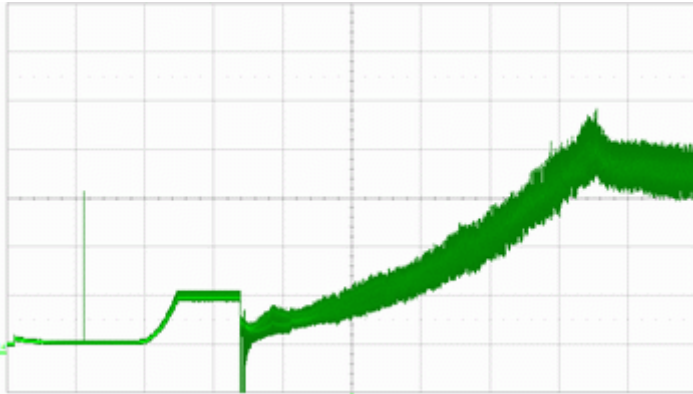
Start-up current at 24 V; 0,5A/div; 2s/div
